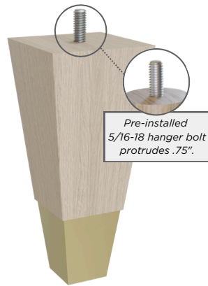
w/SB Slipper Cup 0122206-SB6
