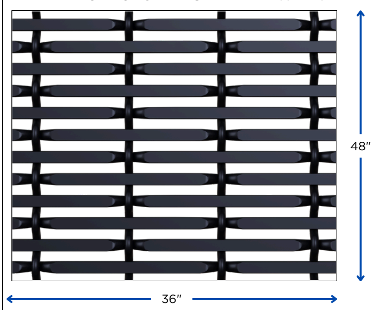
#226 1.25" STRAIGHT FLAT WEAVE
