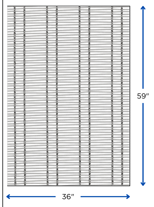
#226 1.25" STRAIGHT FLAT WEAVE
